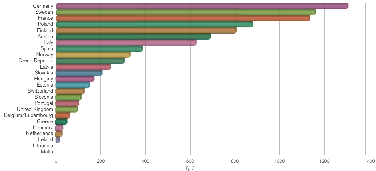
Carbon stock in wood biomass in European forests
