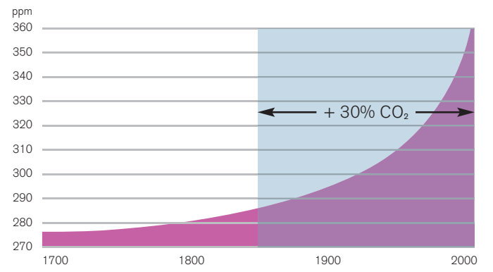
The increasing concentration of CO 2 in the atmosphere
