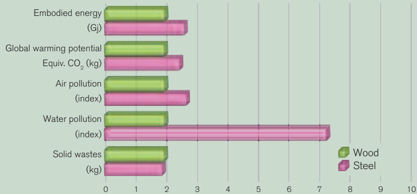
Environmental impacts of wood house vs steel house
