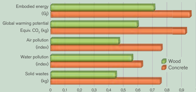
Environmental impacts of wood house vs concrete house
