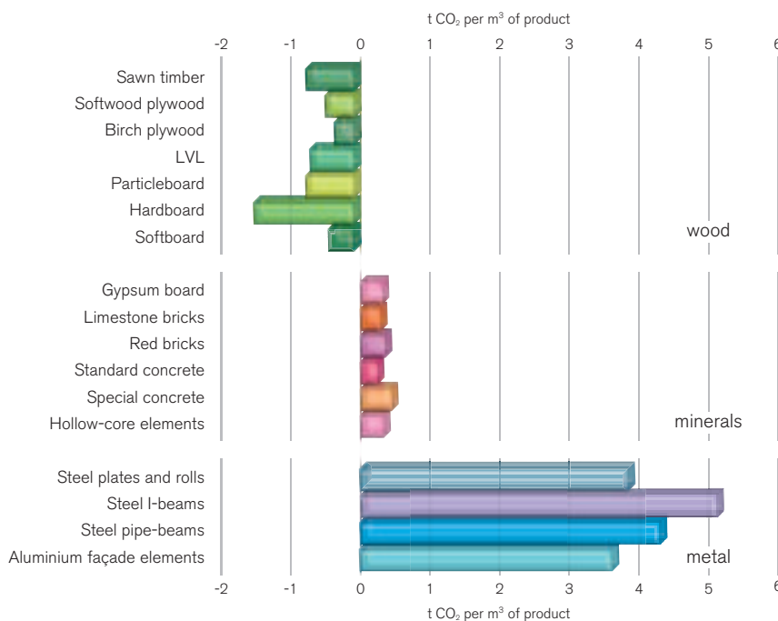
Net CO 2 lifecycle emissions
