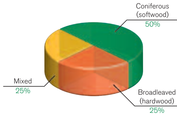
The composition of EU 27 forests
